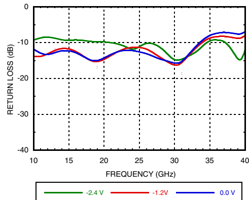
Output Return Loss, Vctl1 = Vctl2
